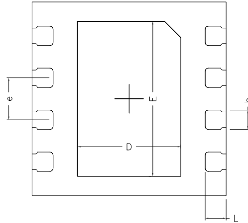
BOTTEM VIEW
