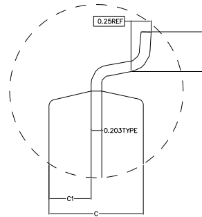
DETAIL E
