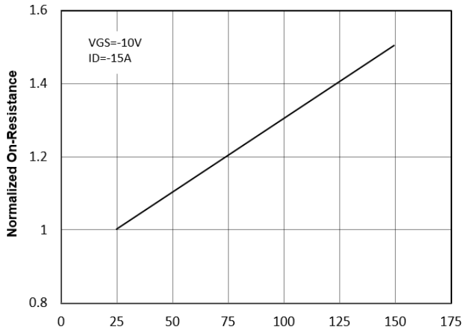
Figure13: Tj Junction Temperature (°C)
